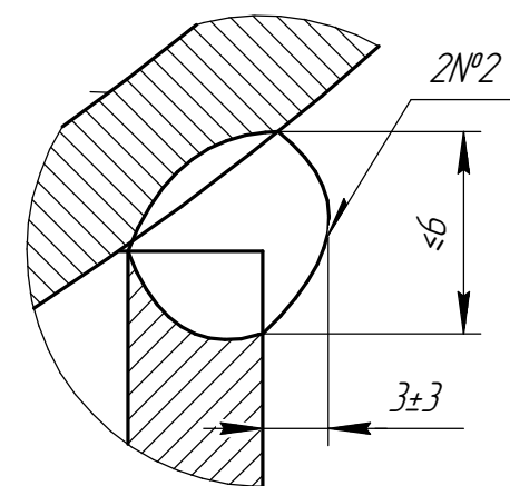
A(4:1)
